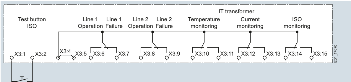
Circuit diagram of 7LQ3361 and 7LQ3362 switchover device to test signaling device (e.g. 7LQ3356 or 7LQ3357 test and signaling panels)
